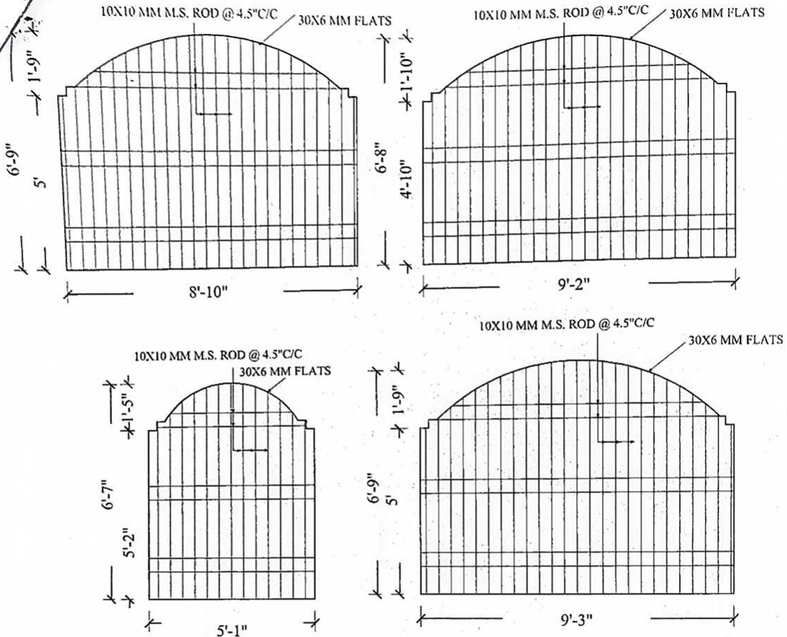
VERANDAH GRILL DETAILS (TYPICAL)
